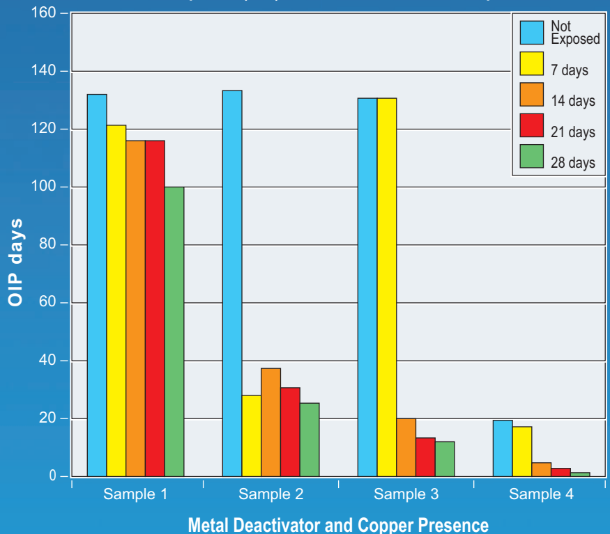
Oxidation induction period (OIP) at 150°C after hot water exposure at 115°C
